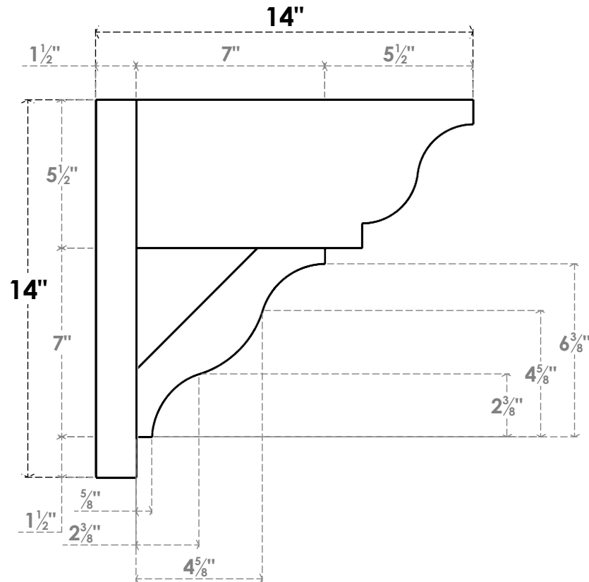
SIDE PROFILE
